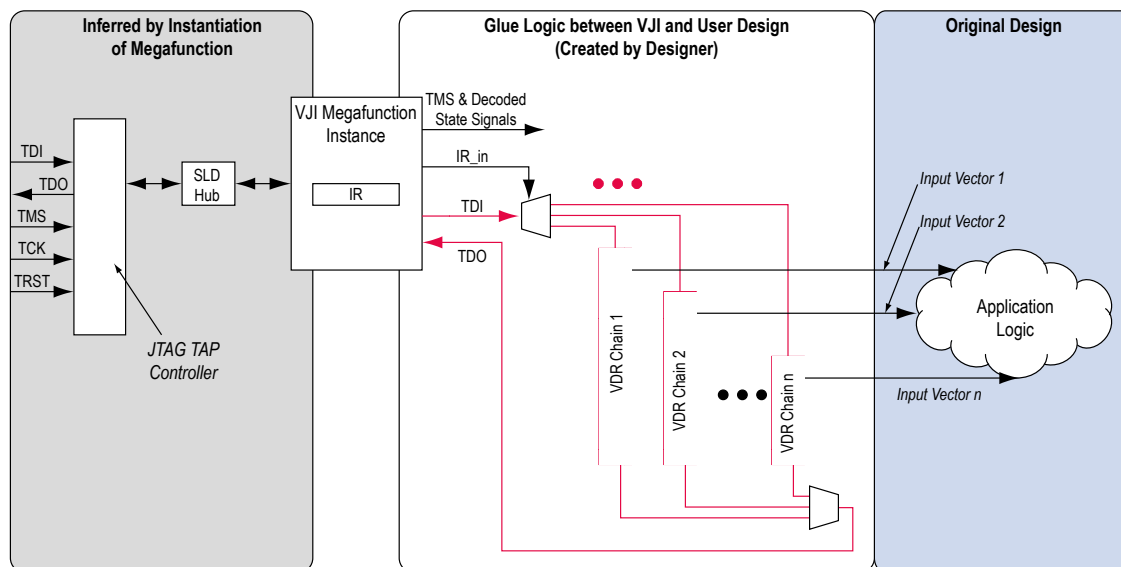
Figure 10: Block Diagram of a Design with a Single Virtual JTAG Instantiation
