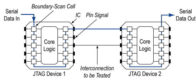
Figure 4: IEEE Std. 1149.1 Boundary-Scan Testing
