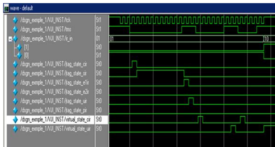
Figure 17: IR Shift Waveform
