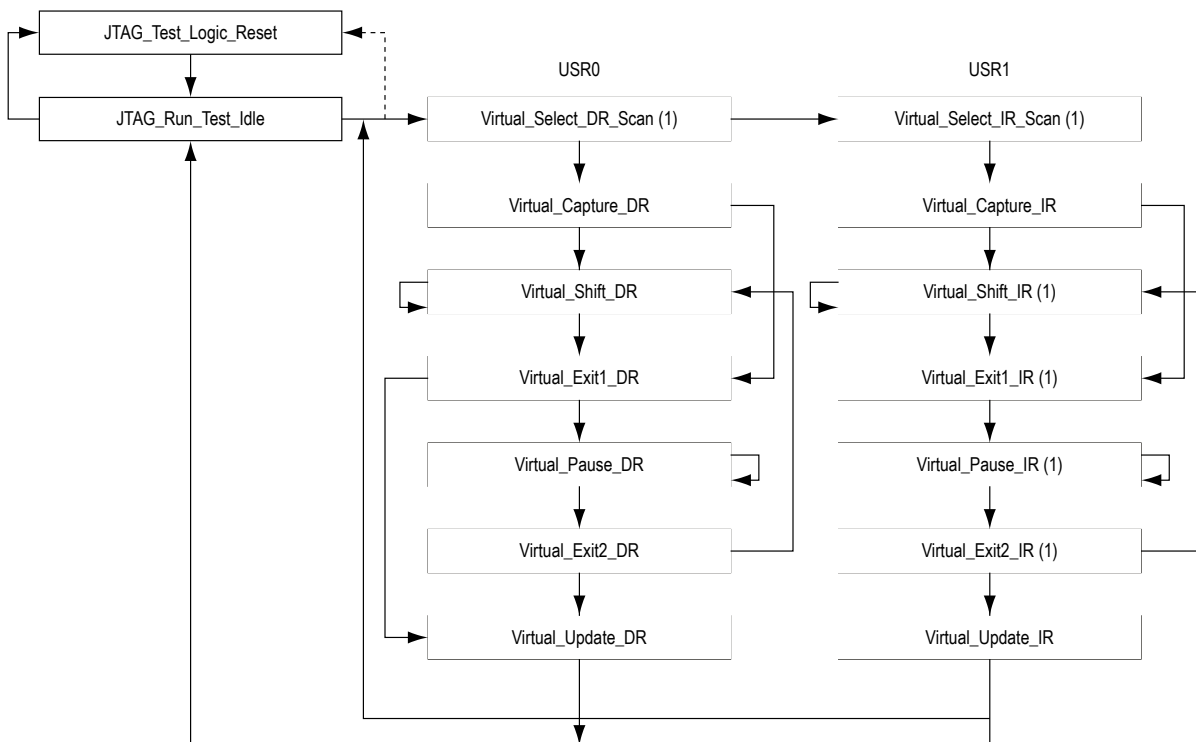
Figure 8: sld_hub Finite State Machine
