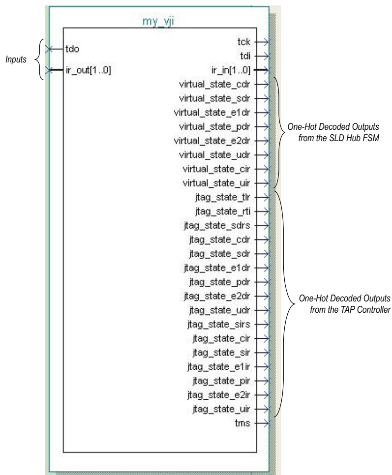
Figure 9: Input and Output Ports of the Virtual JTAG IP Core
