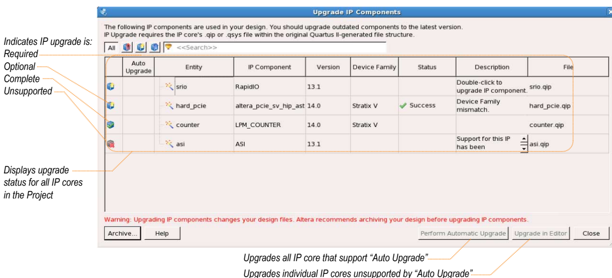
Figure 2: Upgrading Outdated IP Cores
