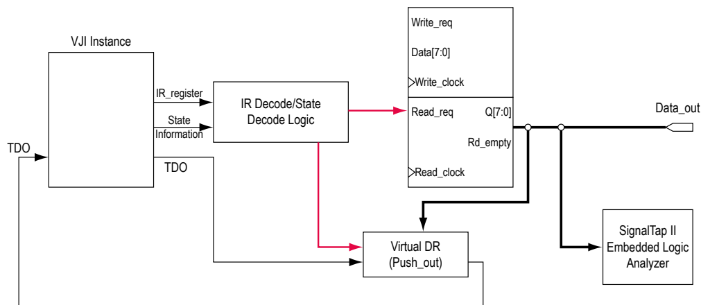
Figure 24: Read Side Logic for DCFIFO Design Example
