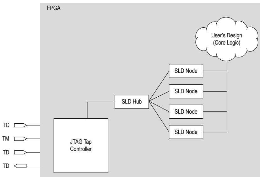
Figure 6: System Level Debugging Infrastructure Functional Model
