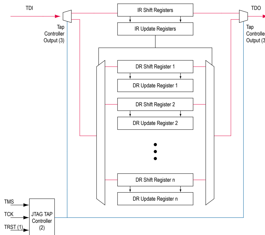
Figure 5: Functional Model of the JTAG Circuitry
