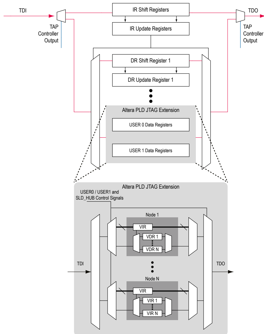
Figure 7: Extension of the JTAG Protocol for PLD Applications
