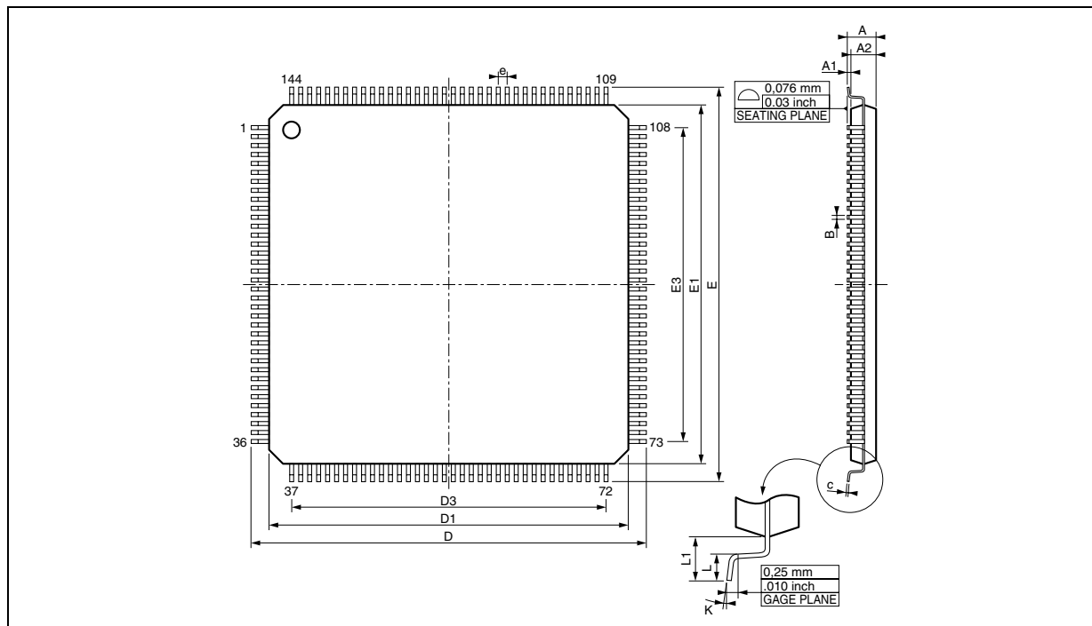
Figure 83 : Package Outline LQFP144 (20 x 20 x 1.40 mm)
