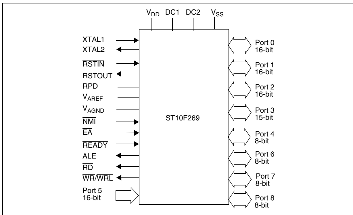
Figure 1 : Logic Symbol
