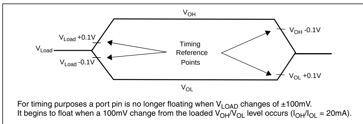
Figure 66 : Float Waveforms
