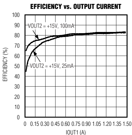
Figure 1. Efficiency vs. Output Current I_{OUT1} , +V_{IN} = 48V
