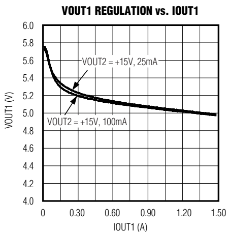
Figure 3. VOUT1 (+5V) Output Voltage Regulation
