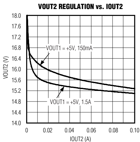
Figure 4. VOUT2 (+15V) Output Voltage Regulation
