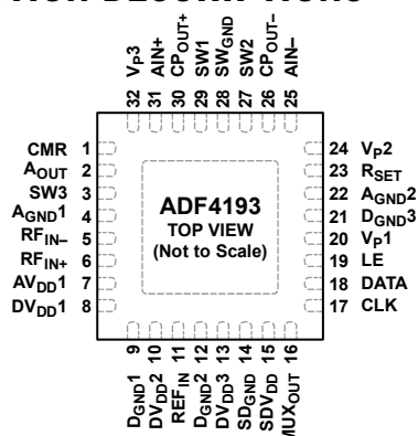
Figure 3. Pin Configuration
