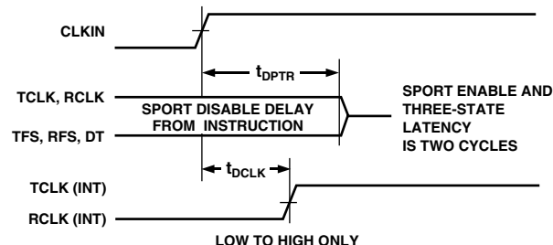
Figure 22. Serial Ports
