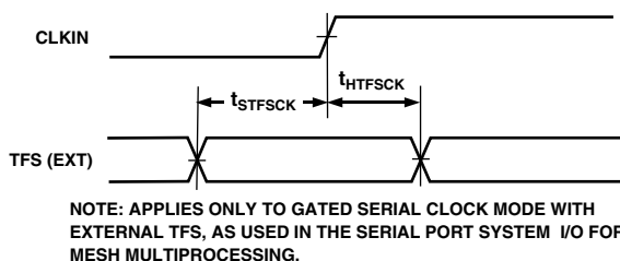
Figure 22. Serial Ports
