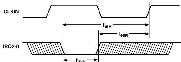
Figure 10. Interrupts
