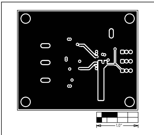
Figure 5. MAX5066 EV Kit PC Board Layout—Internal Layer 3—PGND Layer
