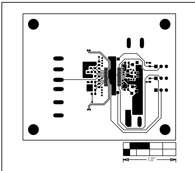
Figure 3. MAX5066 EV Kit PC Board Layout—Component Side
