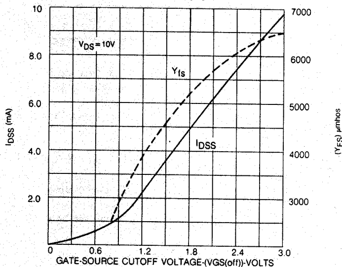
FORWARD TRANSADMITTANCE VS GATE-SOURCE CUTOFF
