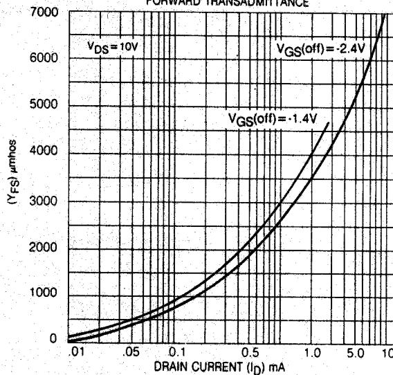
FORWARD TRANSADMITTANCE
