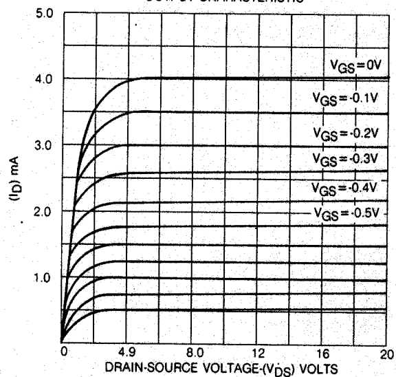
OUTPUT CHARACTERISTIC
