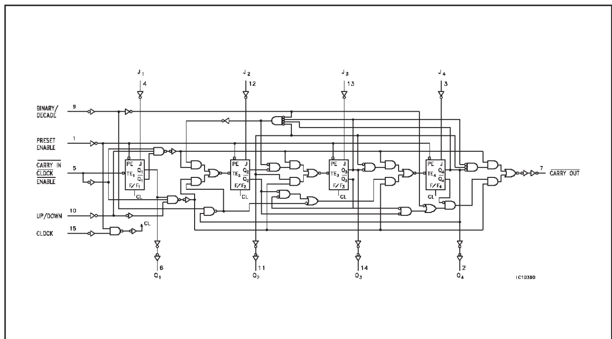
LOGIC DIAGRAM
