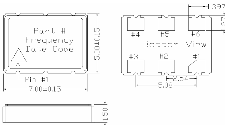
Figure 3. VCC6-QCx Package Drawing
