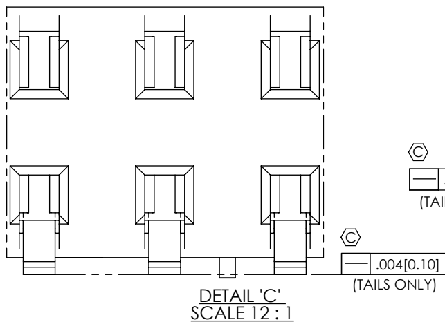
FIG 3 MMS-140-02-XXX-DH-LC SHOWN
