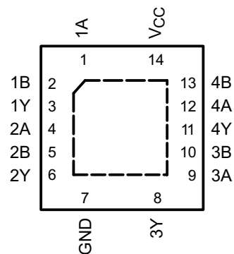
SN74AHC00 . . . RGY PACKAGE (TOP VIEW)
