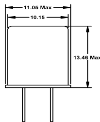
HC49S Resistance Weld
