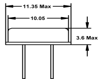
HC49S Resistance Weld
