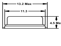
HC49SD Surface Mount
