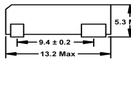
FPX Surface Mount
