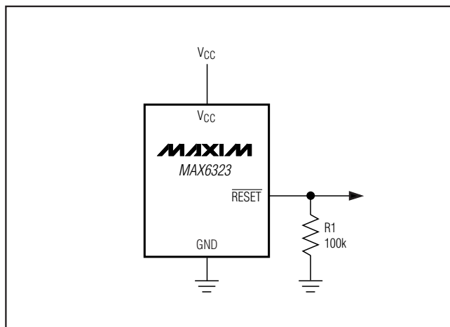
Figure 6. \overline{\text{RESET}} Valid to V_{\text{CC}} = Ground Circuit
