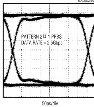
ELECTRICAL EYE DIAGRAM
