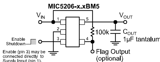
SOT-23-5 Fixed Voltage Application
