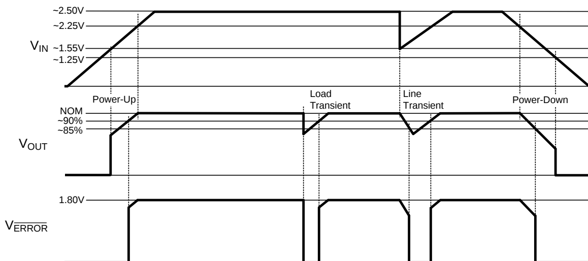
Figure 23. \overline{ERROR} Flag Operation, see Typical Application
