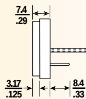
Window Mount Side View
