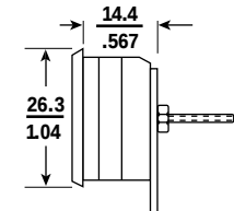
Backlit Bezel Mount Side View
