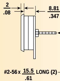
Bezel Mount Side View
