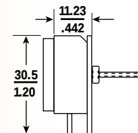
Backlit Window Mount Side View
