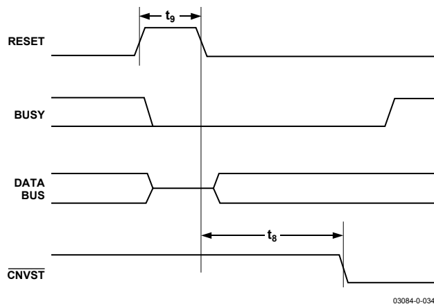
Figure 28. RESET Timing
