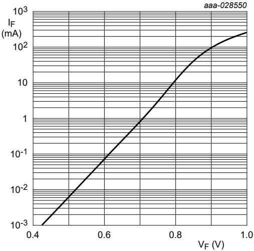
Fig. 2. Forward current as a function of forward voltage; typical values (BZX84J-B/C2V4-Q)
