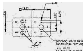
RS 76M, keyboard fully illuminated
