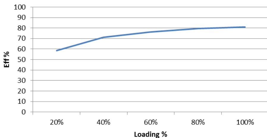
AM1D-1512SZ Efficiency vs. Loading
