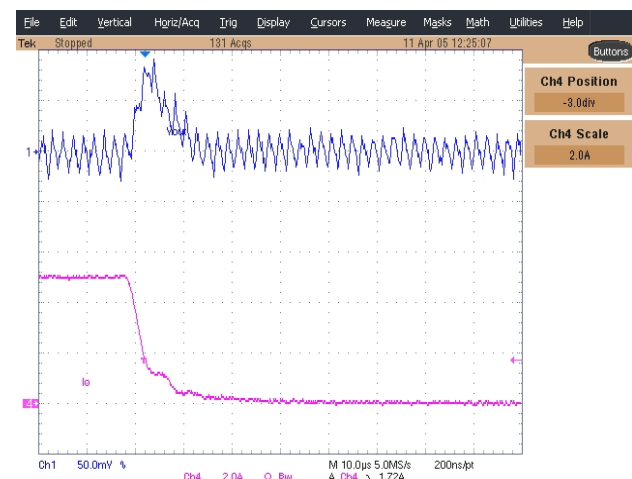
Figure 21 - Load Transient (5-0A) Ch1: Vout, Ch4: Step Load Current
