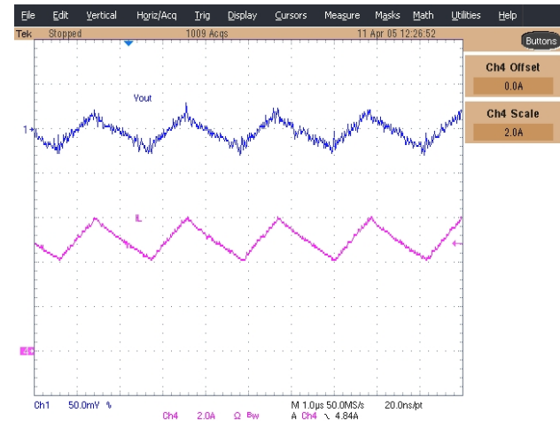
Figure 19 - Output Voltage Ripple Ch1: Vout, Ch4: Inductor Current I_{Load}=5A
