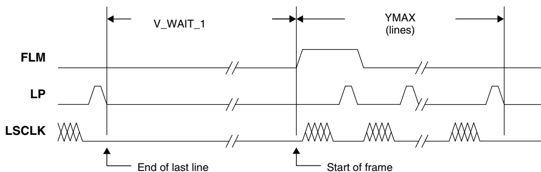
Figure 62-42. Vertical Sync Pulse Timing in Passive Mode
