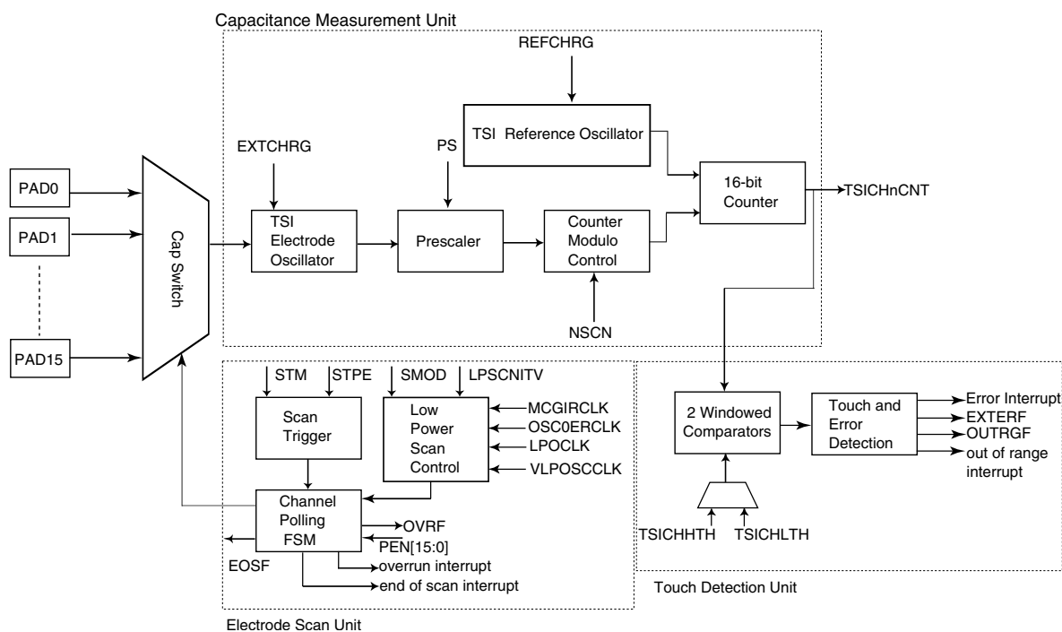
Figure 61-3. TSI block diagram
