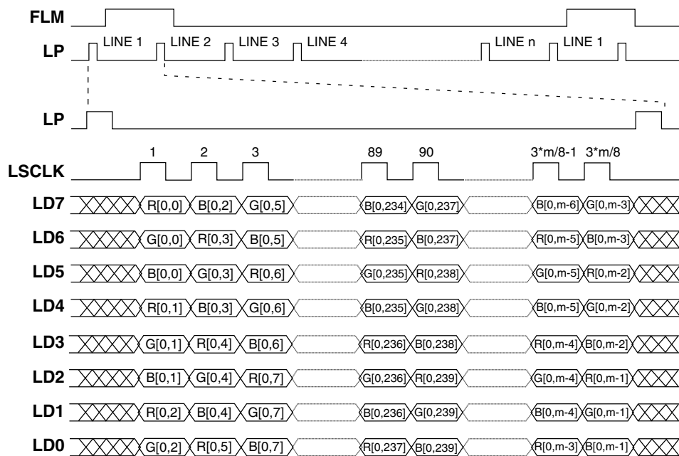
Figure 62-34. LCDC Interface Timing for 8-bit Data Passive Matrix Color Panels
