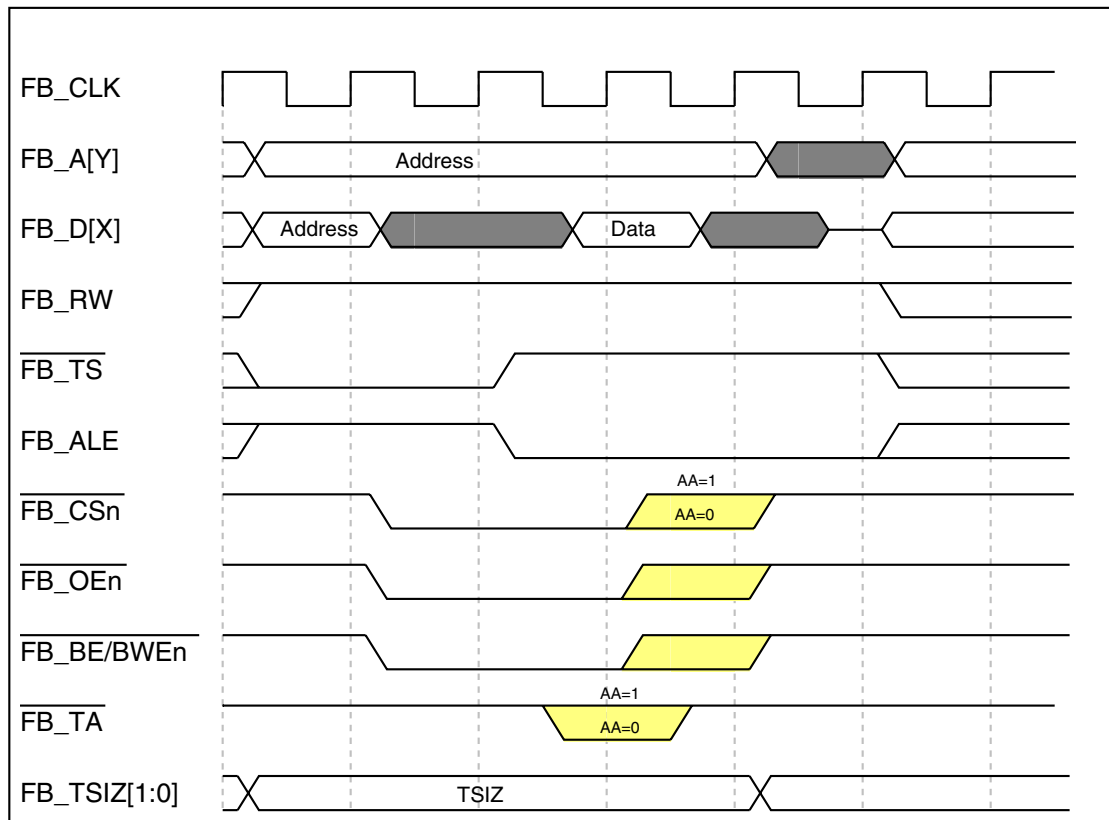
Figure 33-53. Read-Bus Cycle with CSCRn[EXTS] = 1 (One Wait State)
