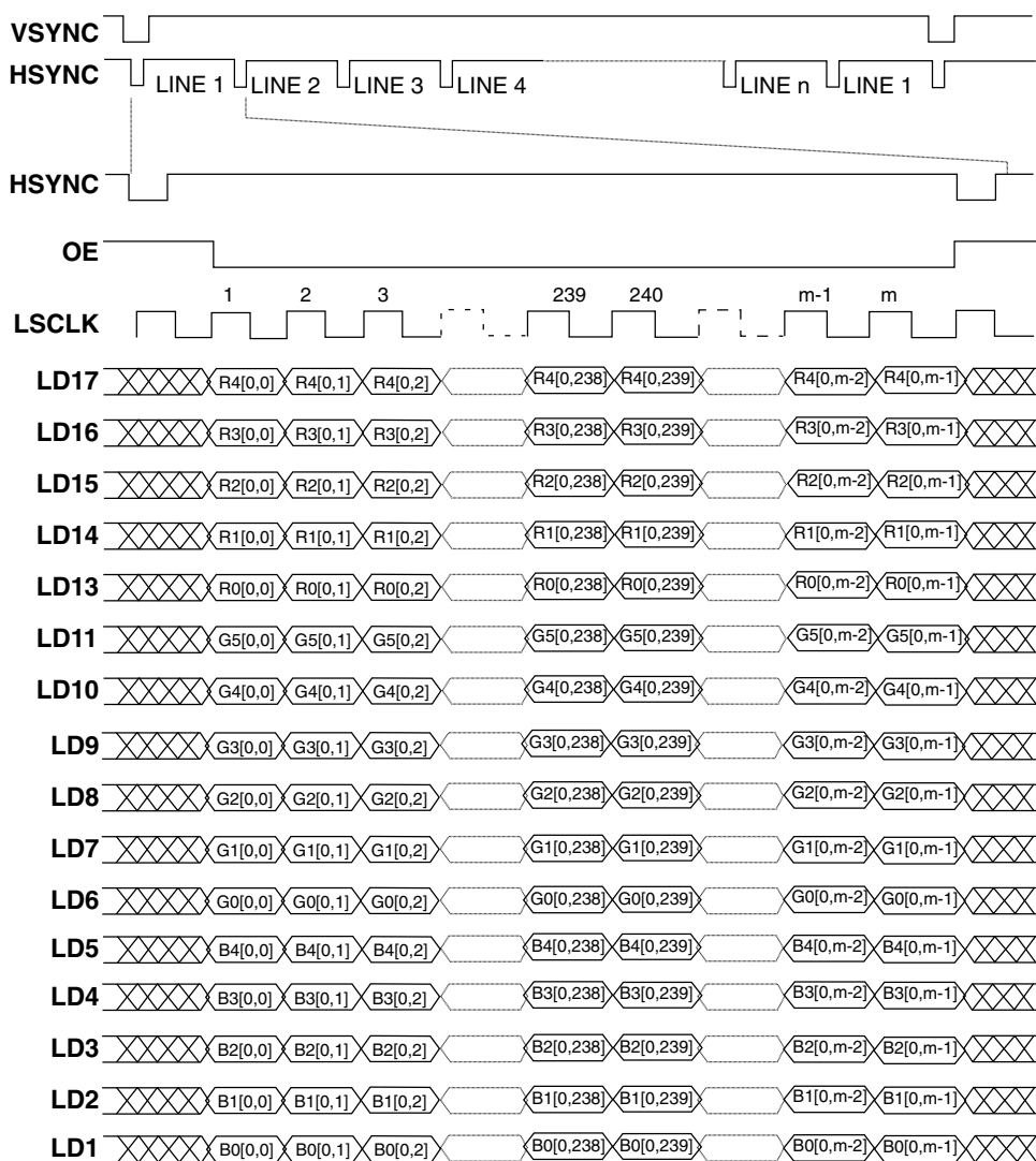
Figure 62-35. LCDC Interface Timing for 16 bpp Active Matrix Color Panels
