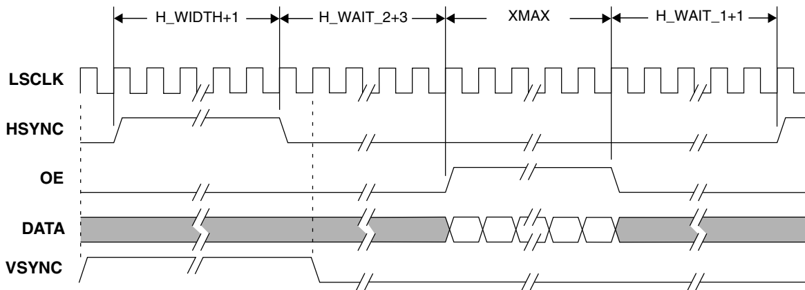
Figure 62-39. Horizontal Sync Pulse Timing in TFT Mode
