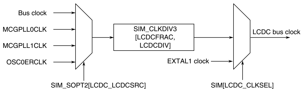
Figure 5-15. LCD controller clock generation
