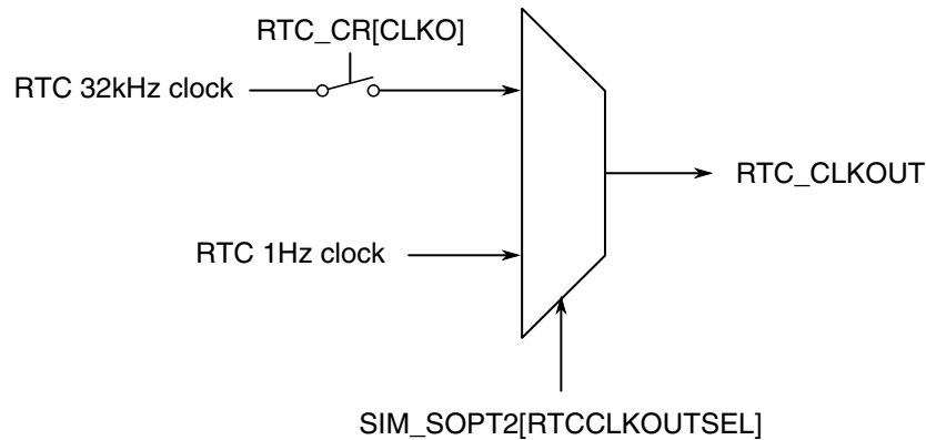
Figure 3-57. RTC_CLKOUT generation
