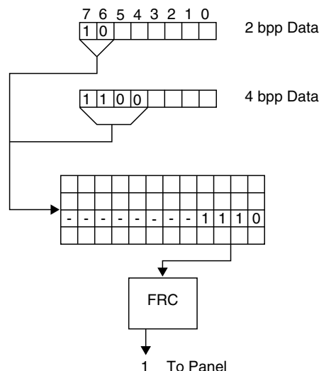
Figure 62-29. Gray-Scale Pixel Generation
