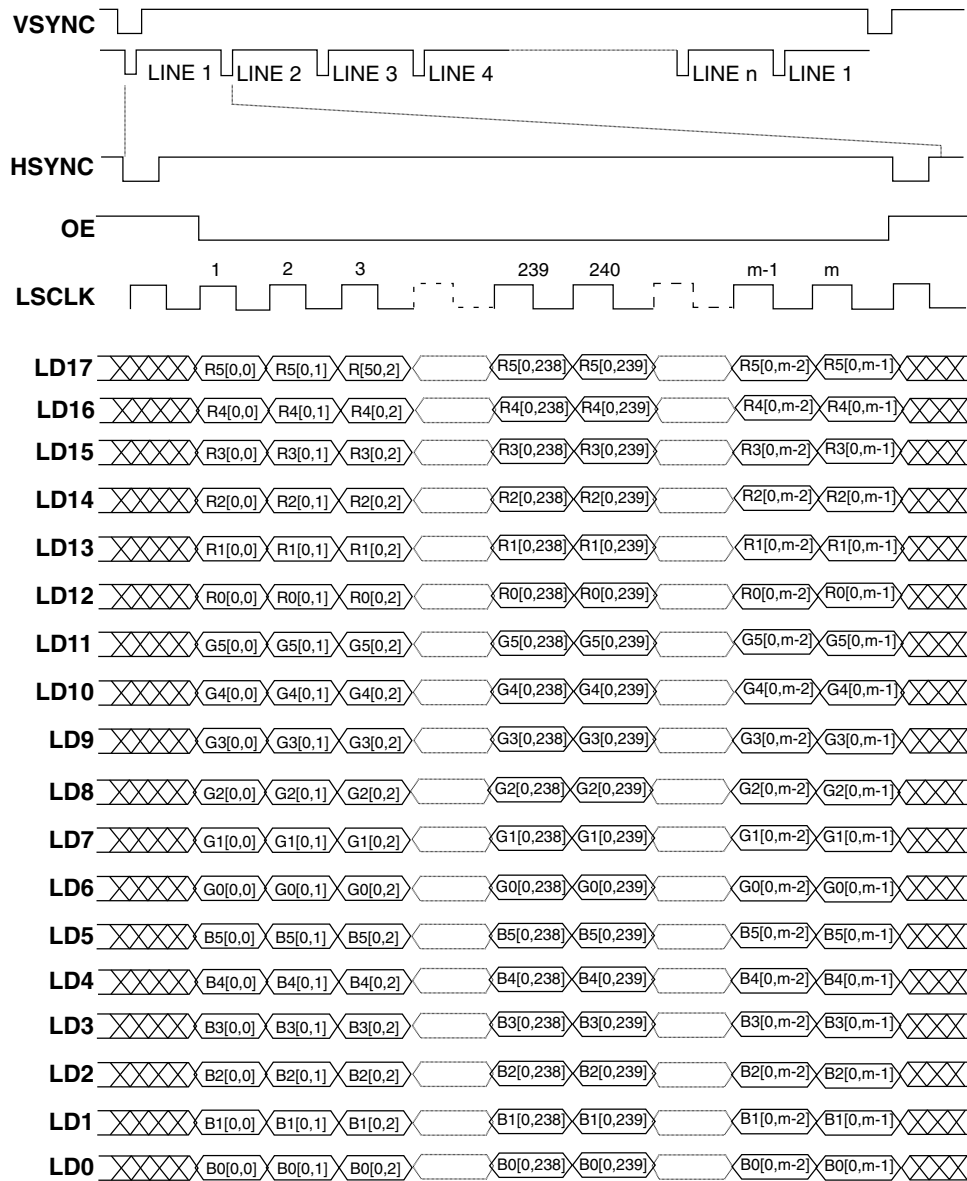
Figure 62-36. LCDC Interface Timing for 18 bpp Active Matrix Color Panels
