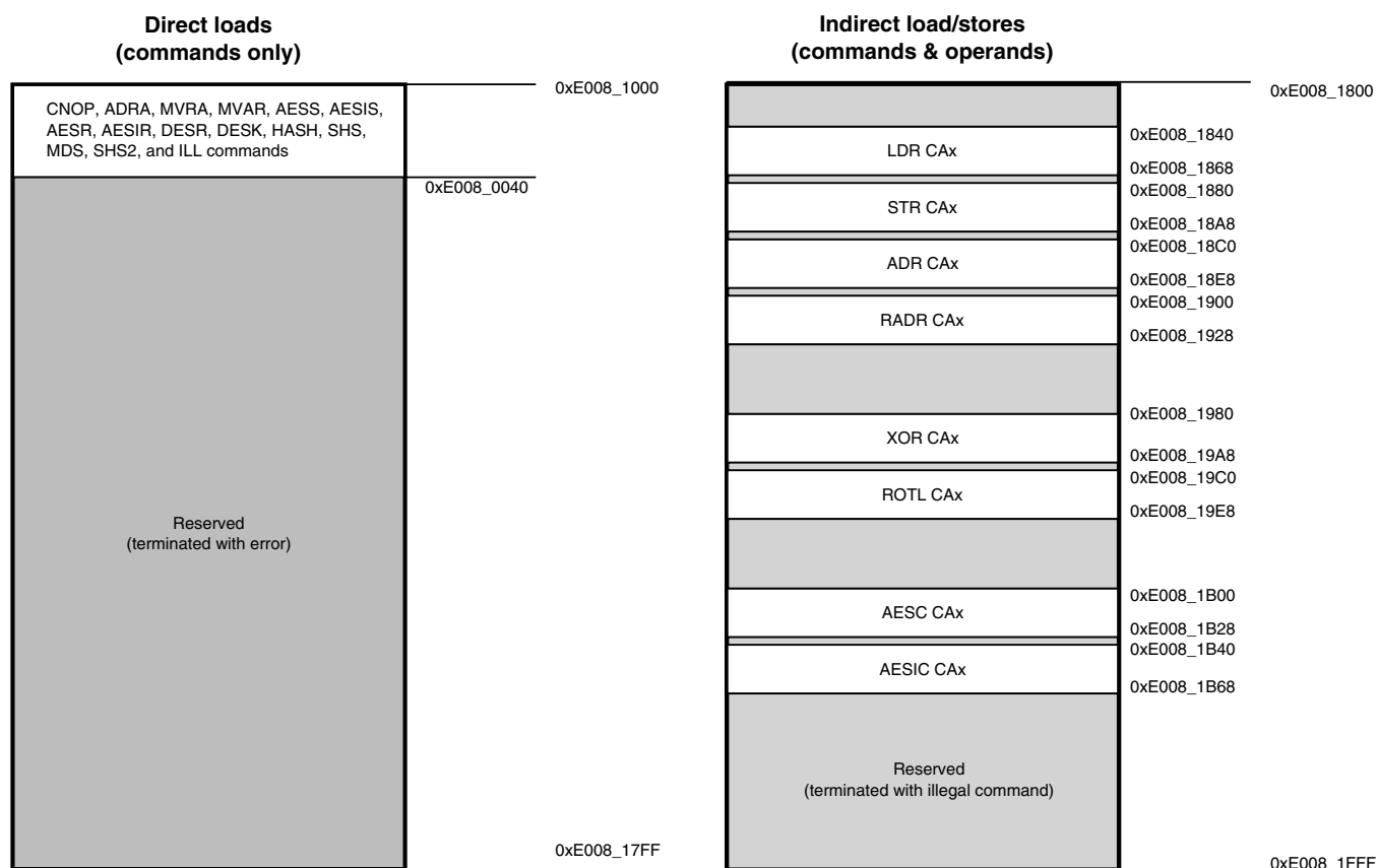
Figure 36-15. MMCAU memory map
