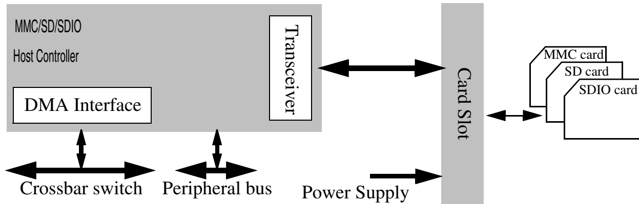
Figure 58-1. System connection of the SDHC
