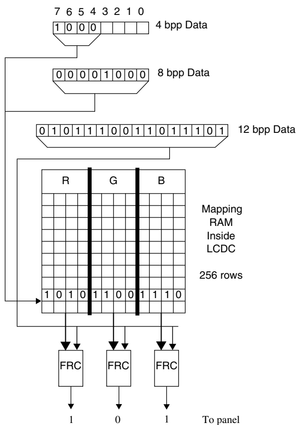
Figure 62-28. Passive Matrix Color Pixel Generation
