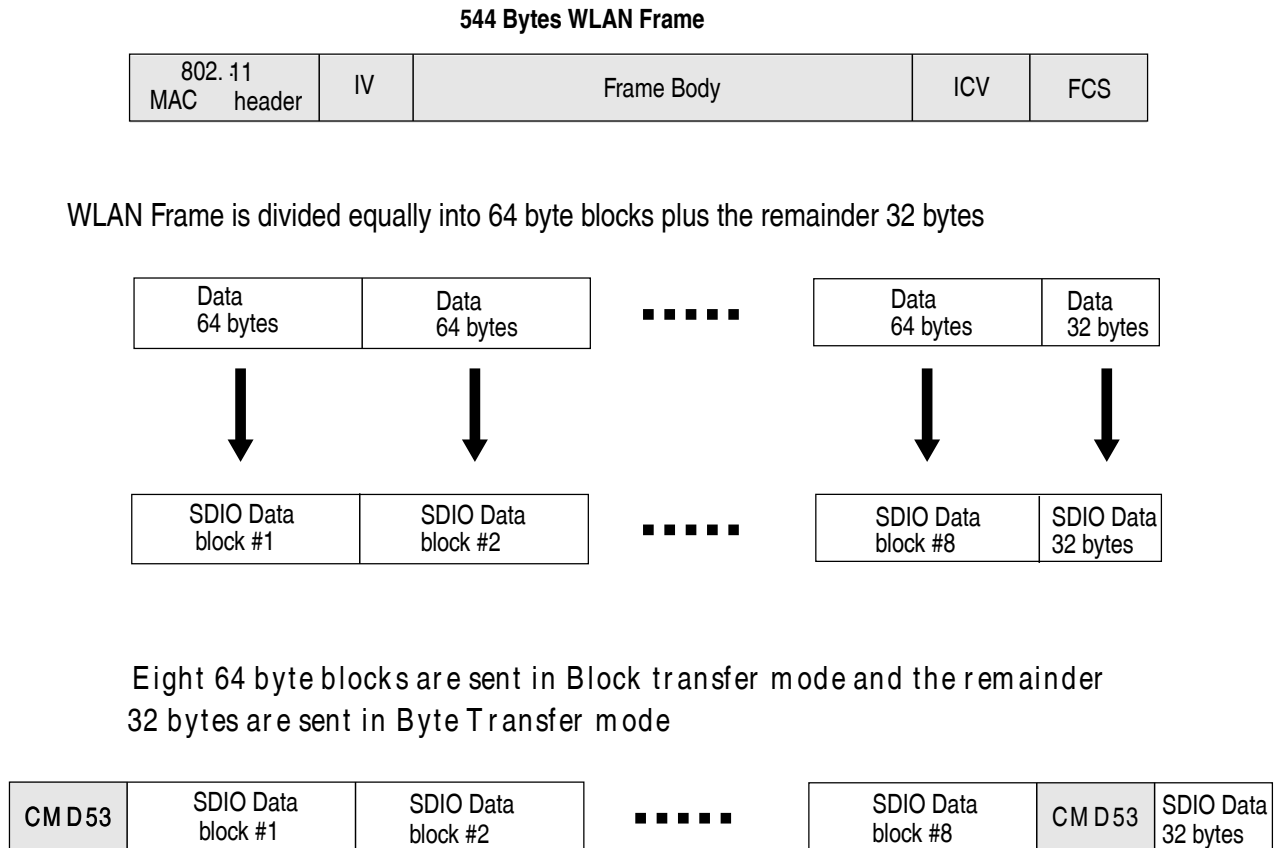
Figure 58-30. Example for dividing large data transfers
