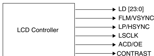
Figure 62-32. LCDC Interface Signals
