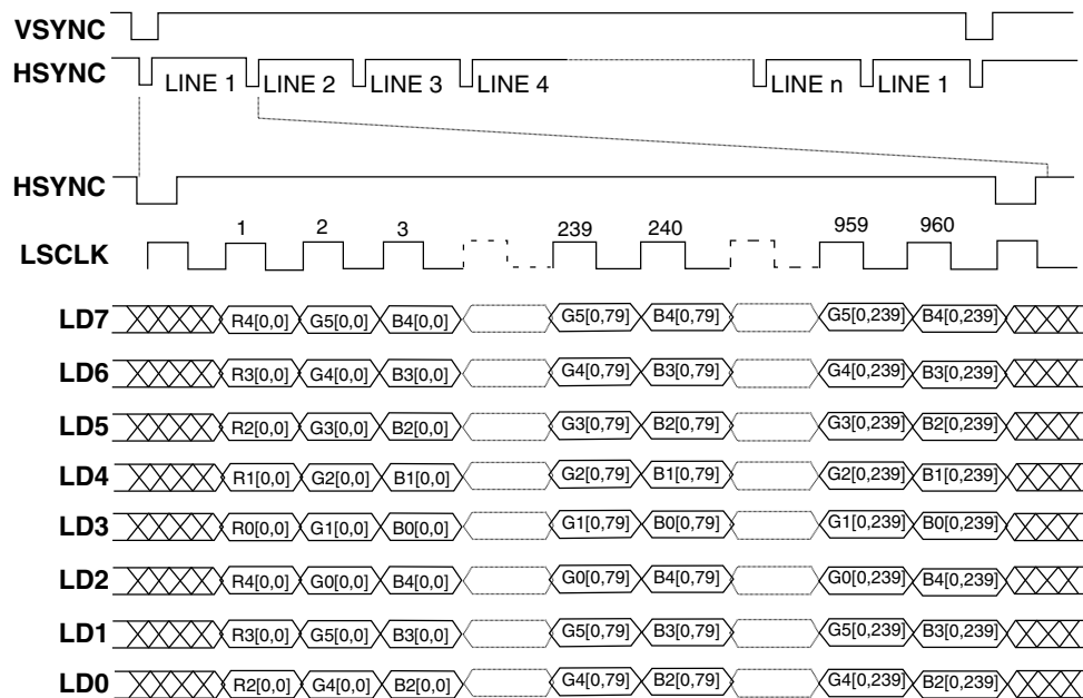
Figure 62-38. LCDC Interface 16-bpp Timing For AUS Mode
