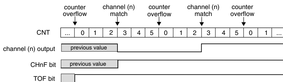
Figure 44-219. Example of the Output Compare Mode when the Match Toggles the Channel Output
