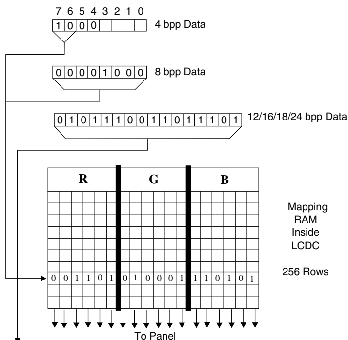
Figure 62-27. Active Matrix Color Pixel Generation
