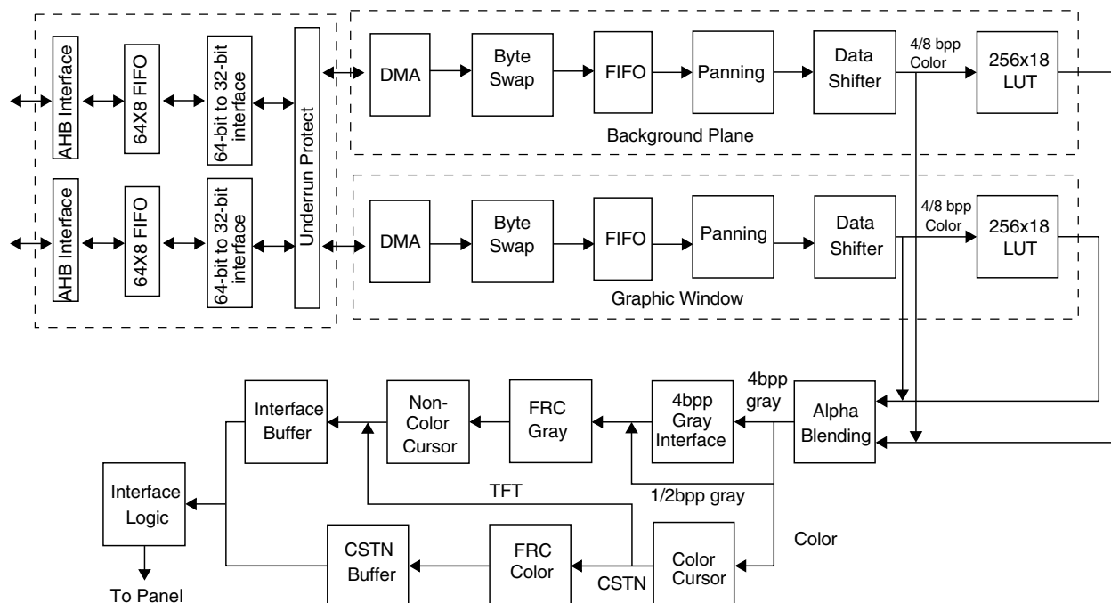
Figure 62-1. LCDC Block Diagram
