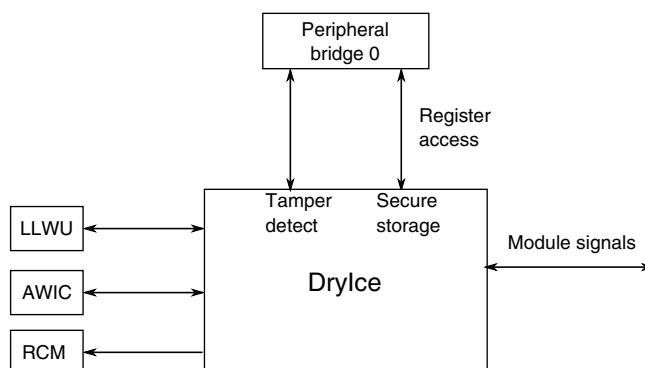
Figure 3-39. DryIce configuration
