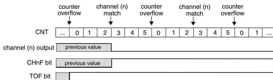
Figure 44-220. Example of the Output Compare Mode when the Match Clears the Channel Output
