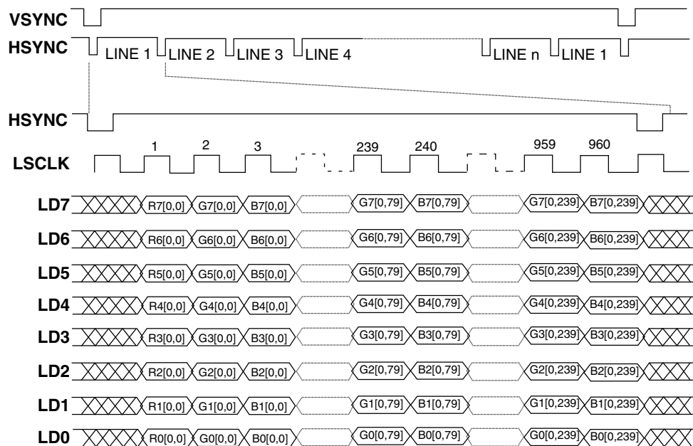
Figure 62-37. LCDC Interface 24-bpp Timing For AUS Mode
