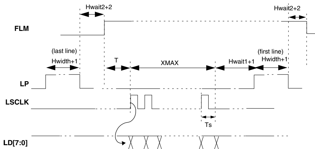
Figure 62-41. Horizontal Sync Pulse Timing in Passive Mode
