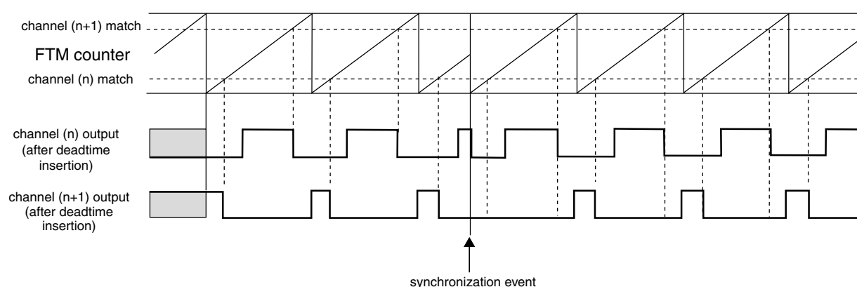
Figure 44-261. FTM Counter Synchronization
