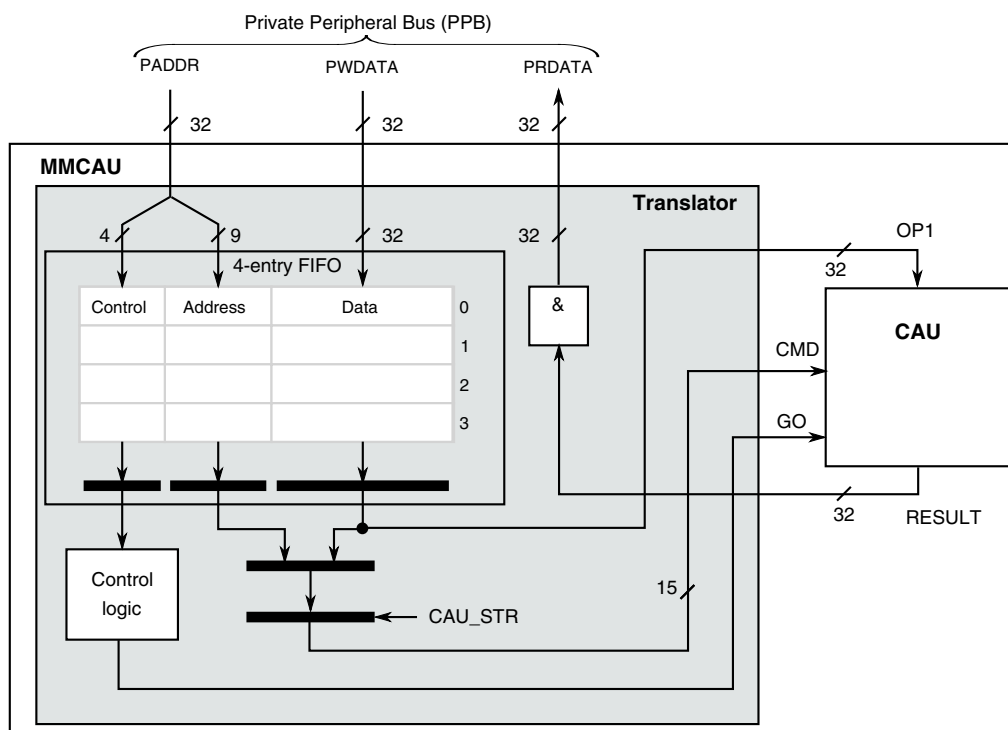
Figure 36-1. MMCAU Block Diagram
