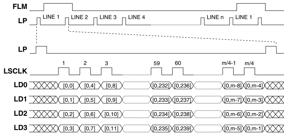
Figure 62-33. LCDC Interface Timing for 4-bit Data Width Gray-Scale Panels
