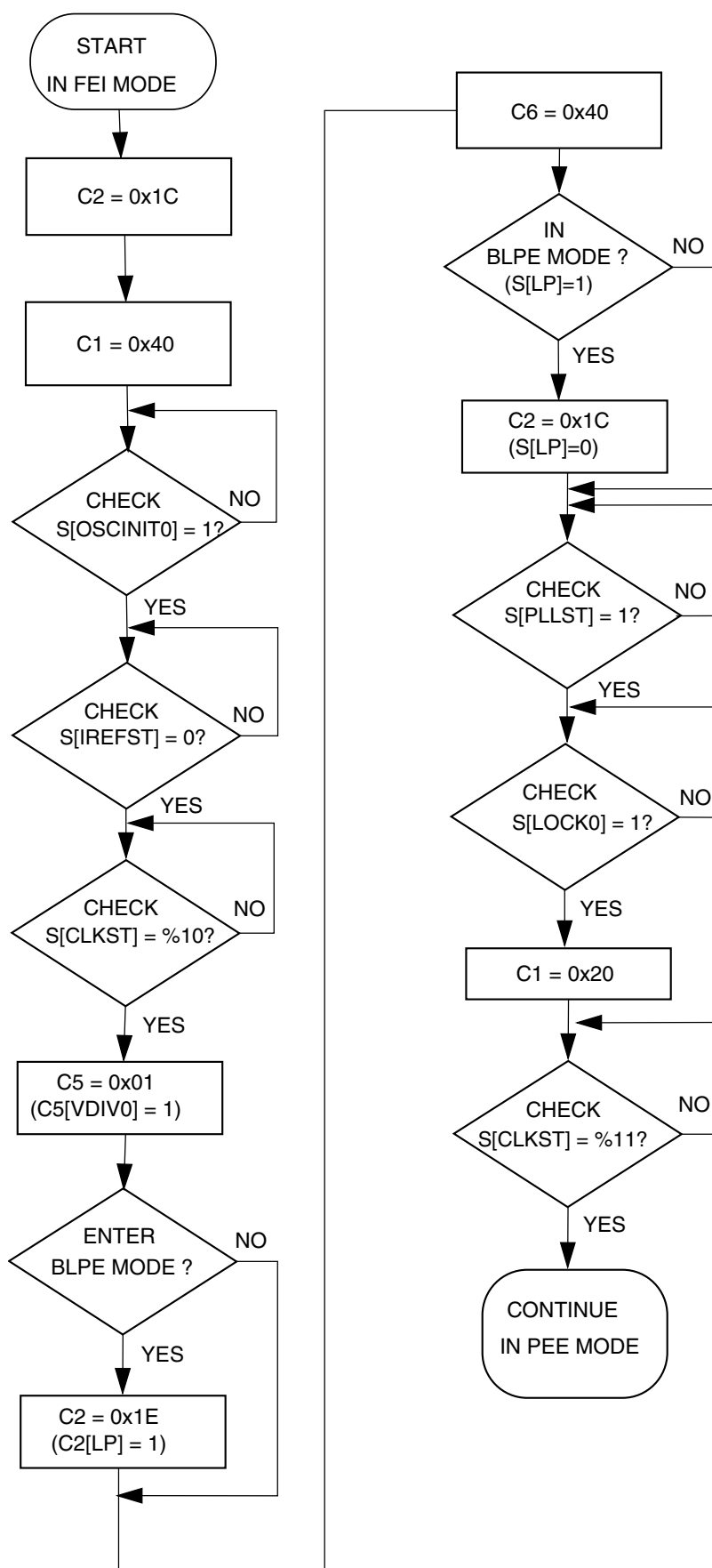
Figure 25-19. Flowchart of FEI to PEE Mode Transition using an 16 MHz crystal K70 Sub-Family Reference Manual, Rev. 2, Dec 2011
