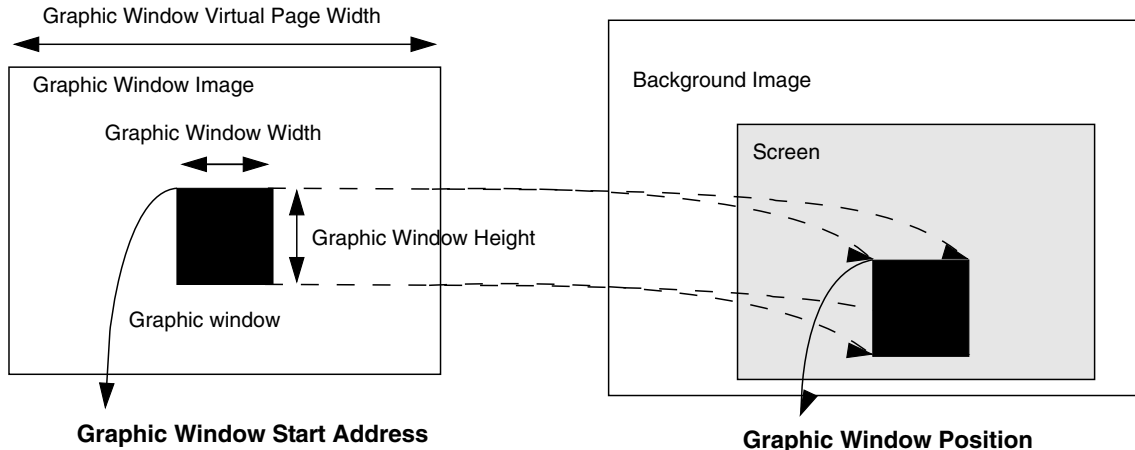
Figure 62-31. Graphic Window on Screen
