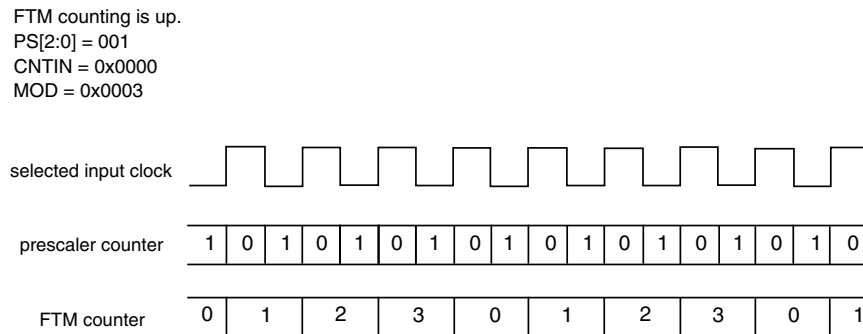
Figure 44-208. Example of the Prescaler Counter
