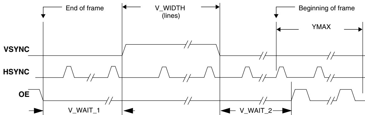
Figure 62-40. Vertical Sync Pulse Timing TFT Mode
