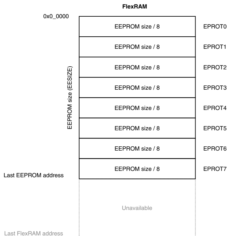
Figure 30-30. EEPROM protection
