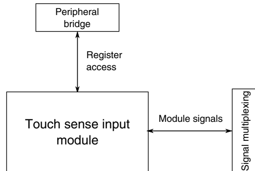
Figure 3-75. TSI configuration
