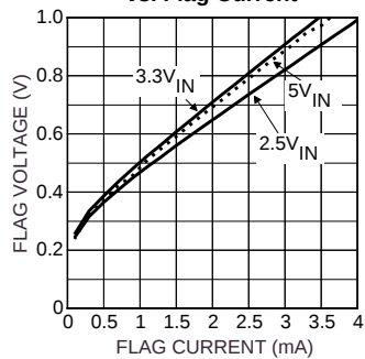
Flag Voltage vs. Flag Current
