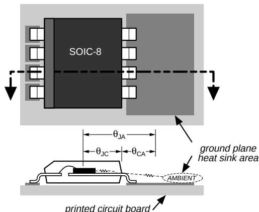
Figure 3. Thermal Resistance
