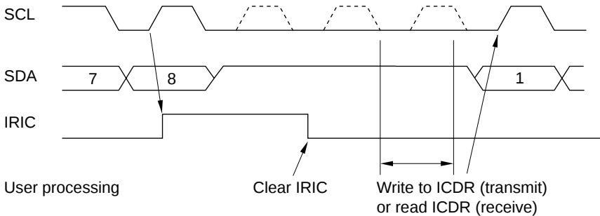
(c) When ACK = 1
