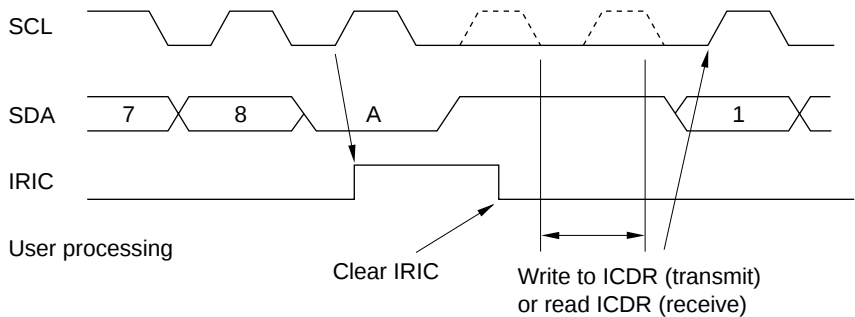
(b) When WAIT = 1 and ACK = 0
