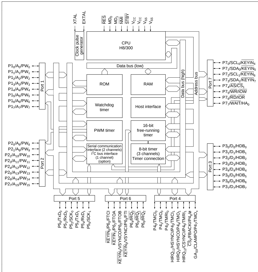
Figure 1-1 Block Diagram
