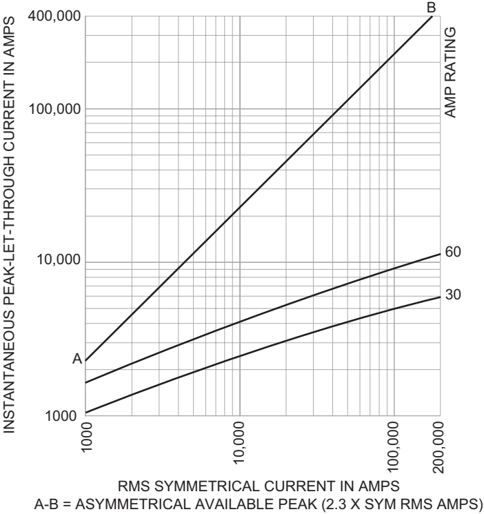
Current-limitation curves — applies only to 600 Vac fuses
