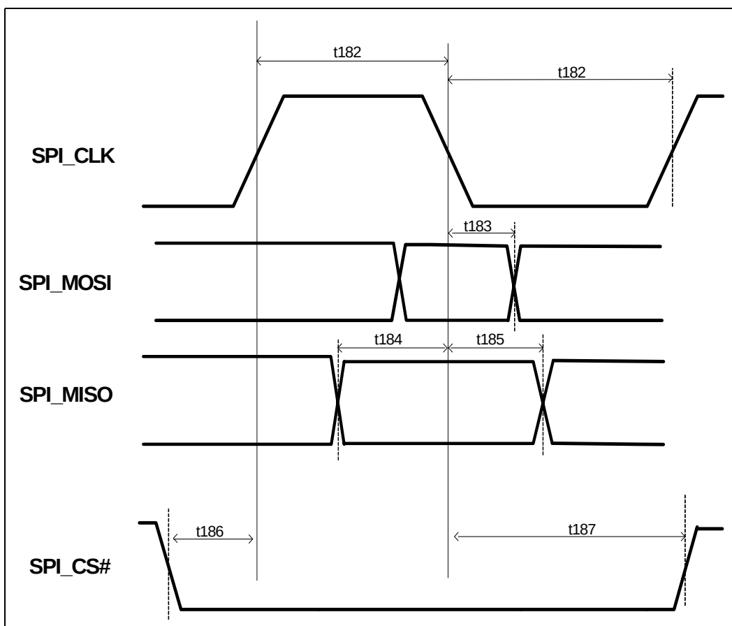
Figure 8-12. SPI Timings
