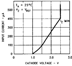
Input Current vs V_Z
