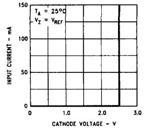
Input Current vs V_Z
