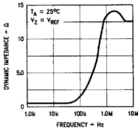
Dynamic Impedance vs Frequency
