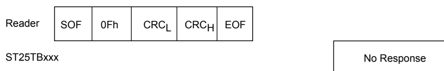
Figure 32. Completion frame exchange between reader and ST25TB04K
