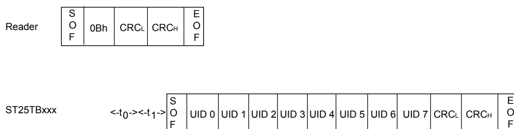
Figure 55. Get_UID frame exchange between reader and ST25TB04K
