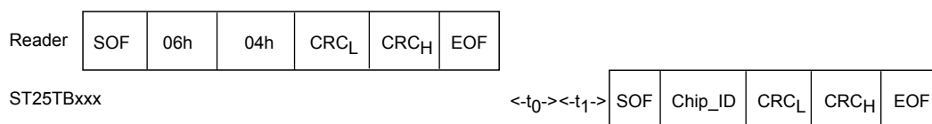
Figure 23. Pcall16 frame exchange between reader and ST25TB04K
