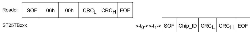
Figure 20. Initiate frame exchange between reader and ST25TB04K
