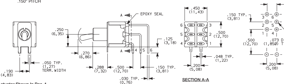
7201MD9AV2BE Vertical Actuation DPDT
