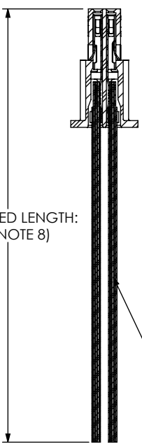
FIG. 1 -S: SINGLE END (SFSD-10-28-XX-XX.XX-S SHOWN)
