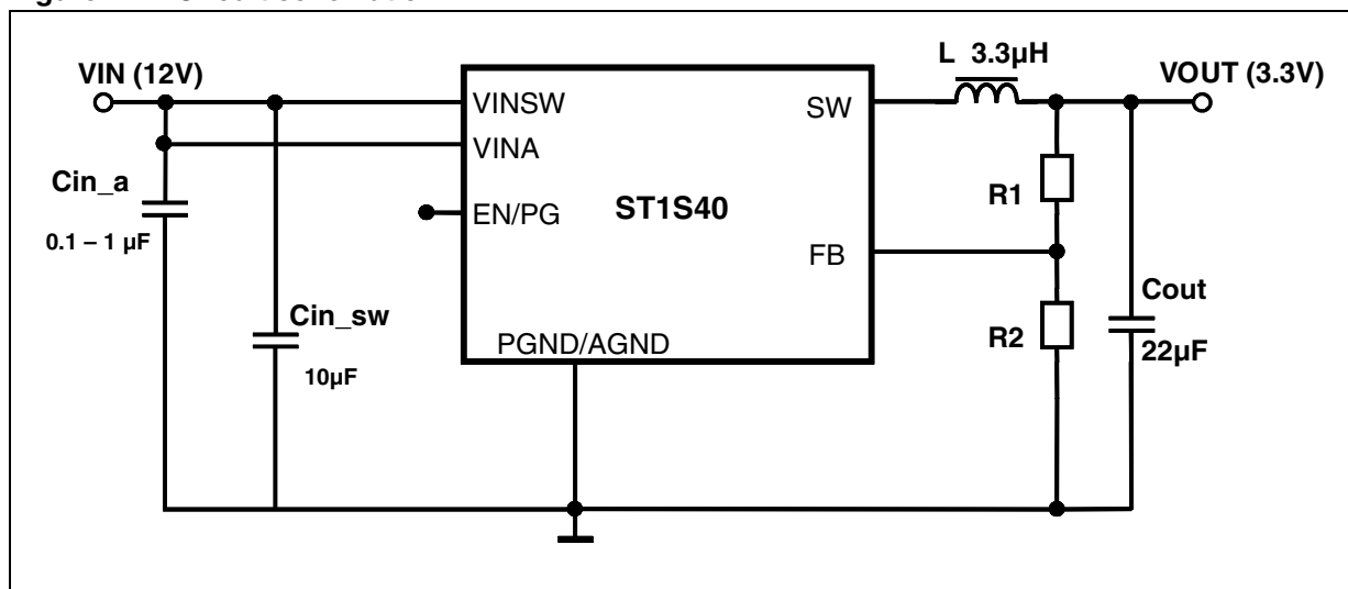
Figure 1. Circuit schematic
