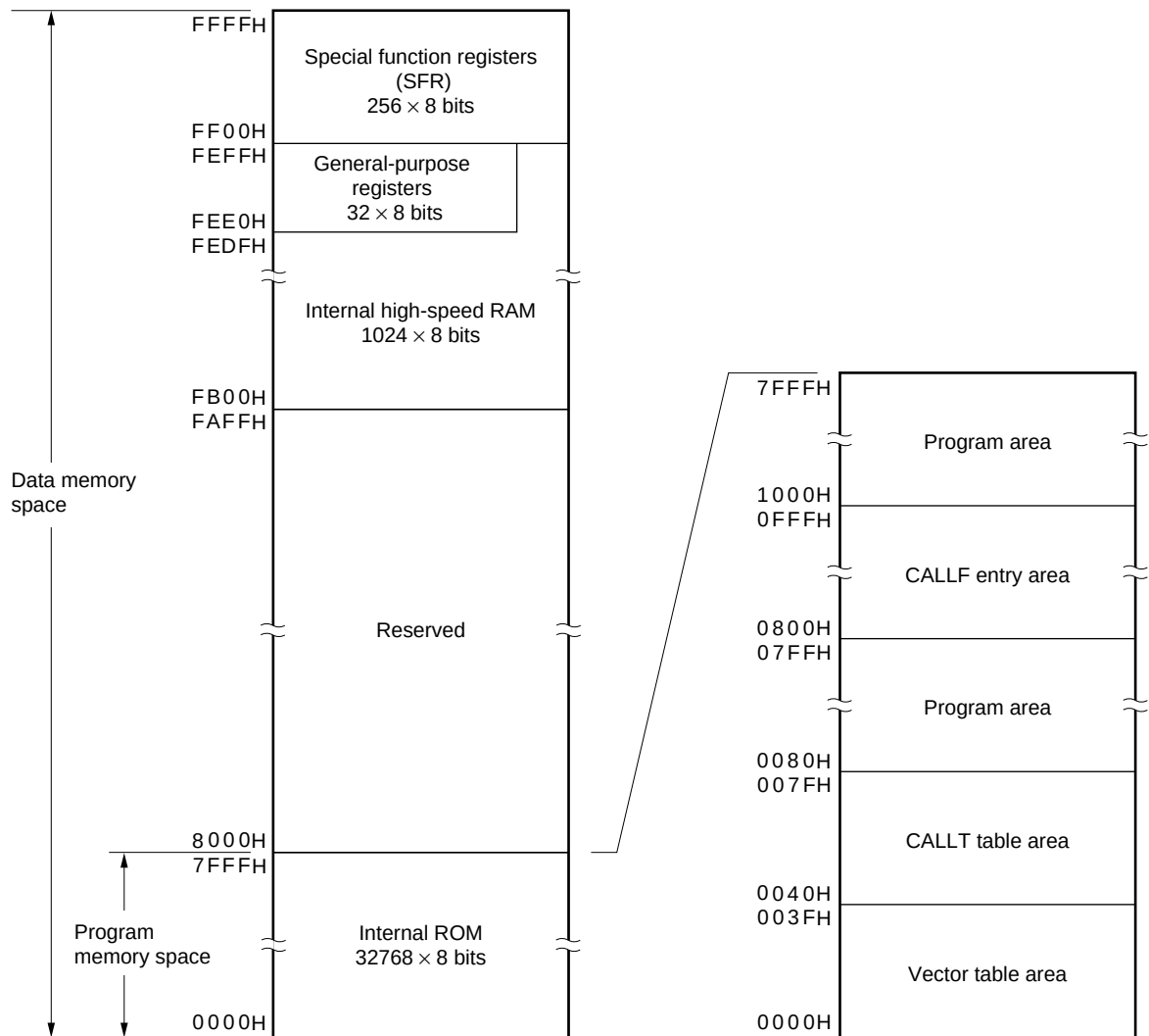
Figure 3-4. Memory Map ( \mu PD780134)
