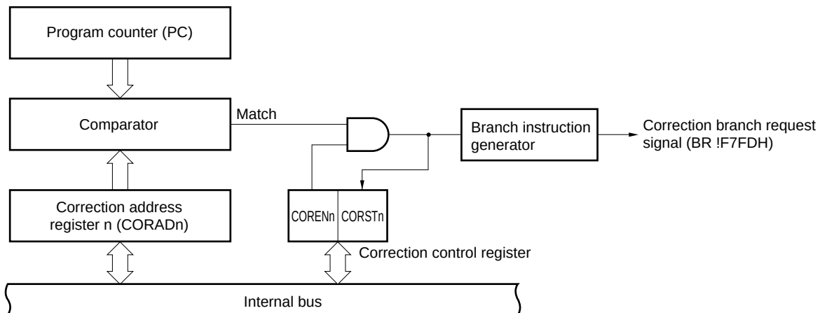
Figure 26-1. Block Diagram of ROM Correction
