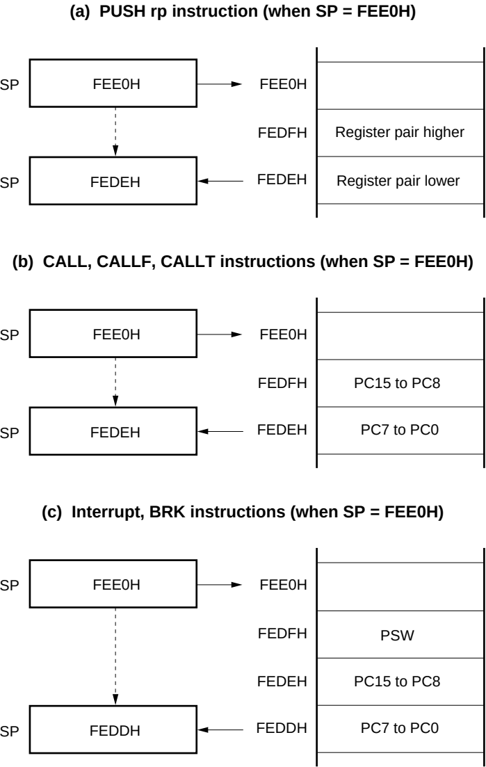
Figure 3-20. Data to Be Saved to Stack Memory
