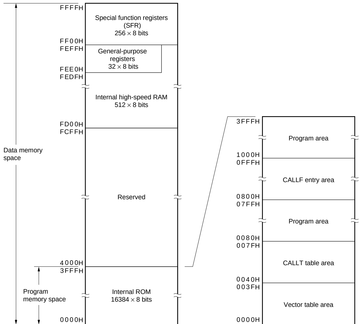
Figure 3-2. Memory Map ( \mu PD780132)
