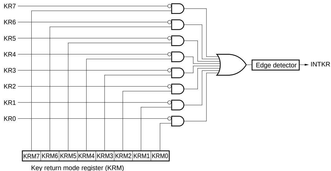
Figure 18-1. Block Diagram of Key Interrupt
