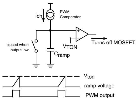
Figure 9. PWM Circuit and Timing Diagram
