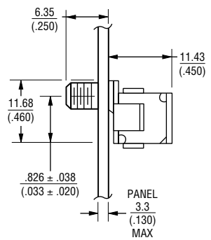
PANEL LAYOUT
