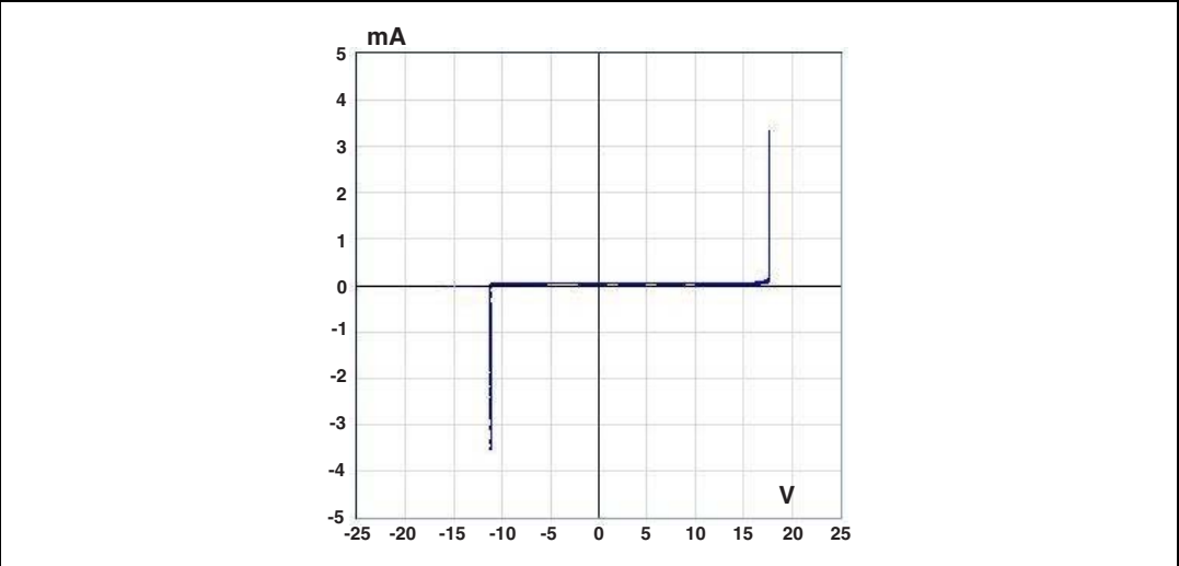
Figure 10. Static characteristic
