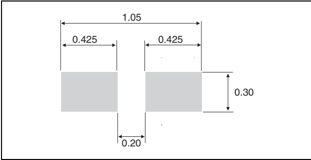
Figure 12. Footprint (dimensions in mm)
