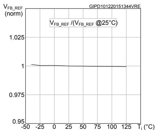
Figure 7. V_{FB\_REF} vs T_J
