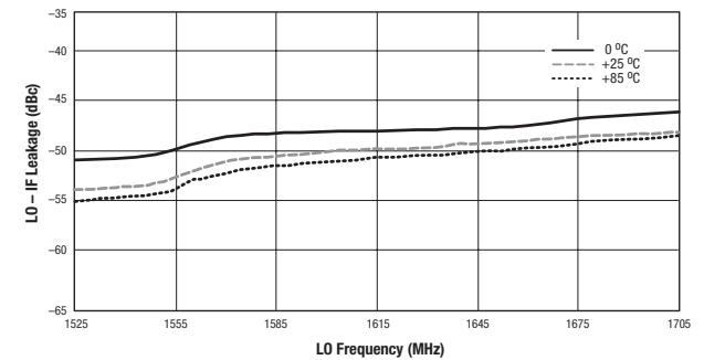
Figure 30. Mixer A LO to IF Leakage vs Frequency and Temperature
