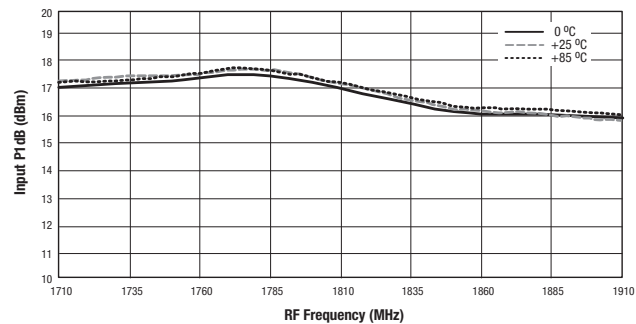
Figure 22. Mixer A Input P1dB vs Frequency and Temperature
