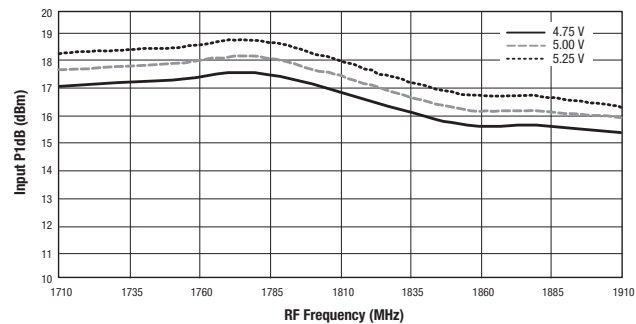
Figure 24. Mixer B Input P1dB vs Frequency and Supply Voltage
