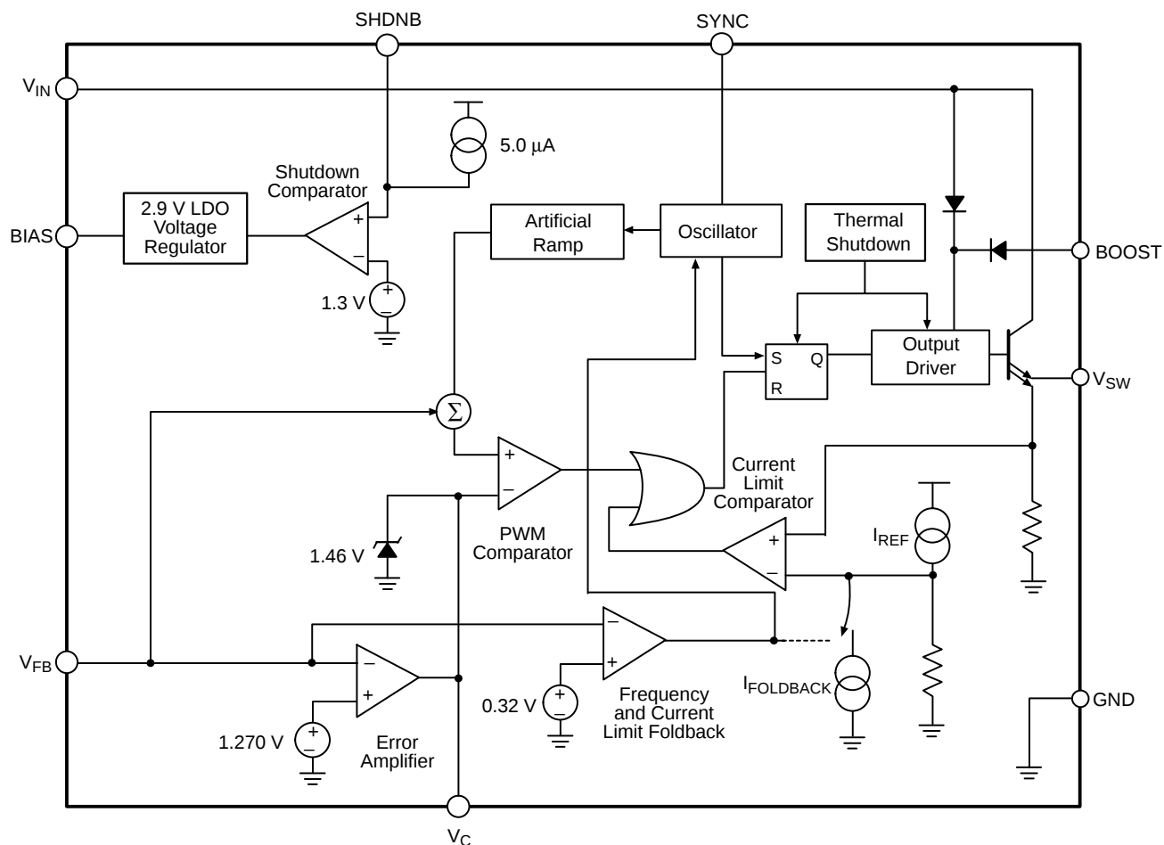
Figure 2. Block Diagram
