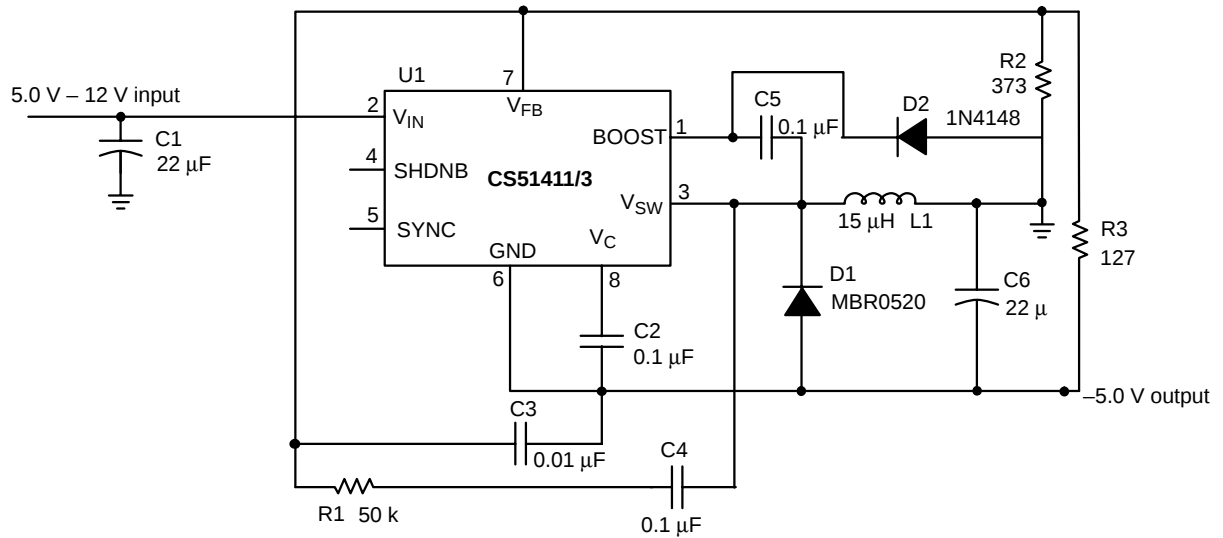
Figure 16. Additional Application Diagram, 5.0 V to -5.0 V/400 mA Inverting Converter
