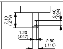
Quick-connect Z
