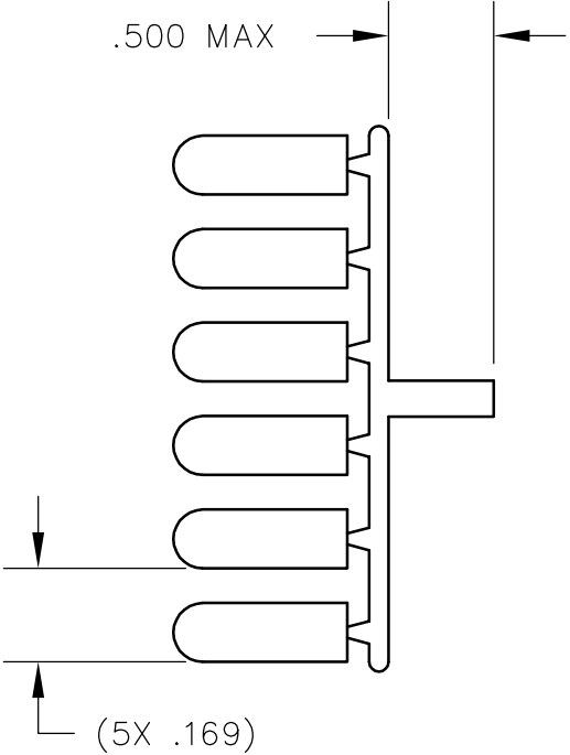
RUNNER CONFIGURATION SCALE - 2:1
