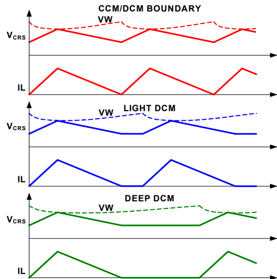
FIGURE 12. PERIOD STRETCHING
