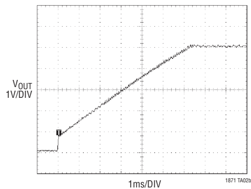
Soft-Start
