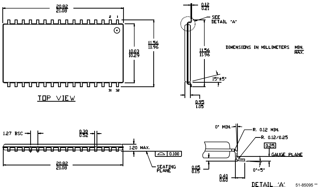
Figure 2. 32-Lead Thin Small Outline Package Type II (51-85095)
