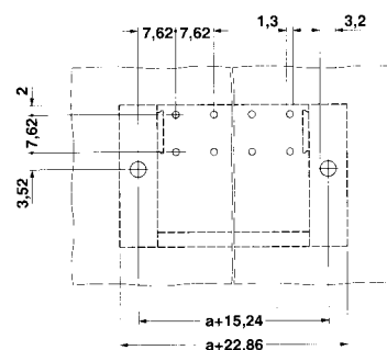
Drilling diagram PC 4/...-G (with BF-PC 4)
