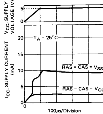
Fig. 21 — CURRENT WAVE FORM DURING POWER UP (ON MEMORY BOARD)
