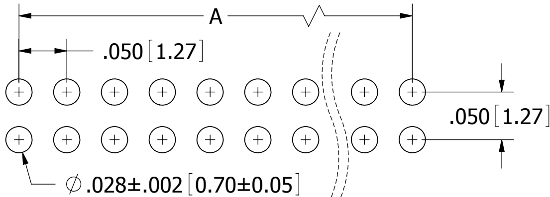
RECOMMENDED PCB HOLE LAYOUT
