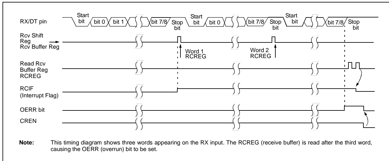
FIGURE 16-5: ASYNCHRONOUS RECEPTION
