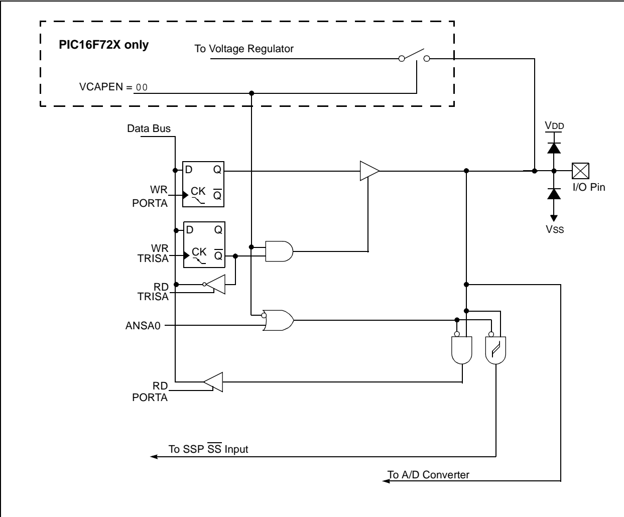
FIGURE 6-1: BLOCK DIAGRAM OF RAO
