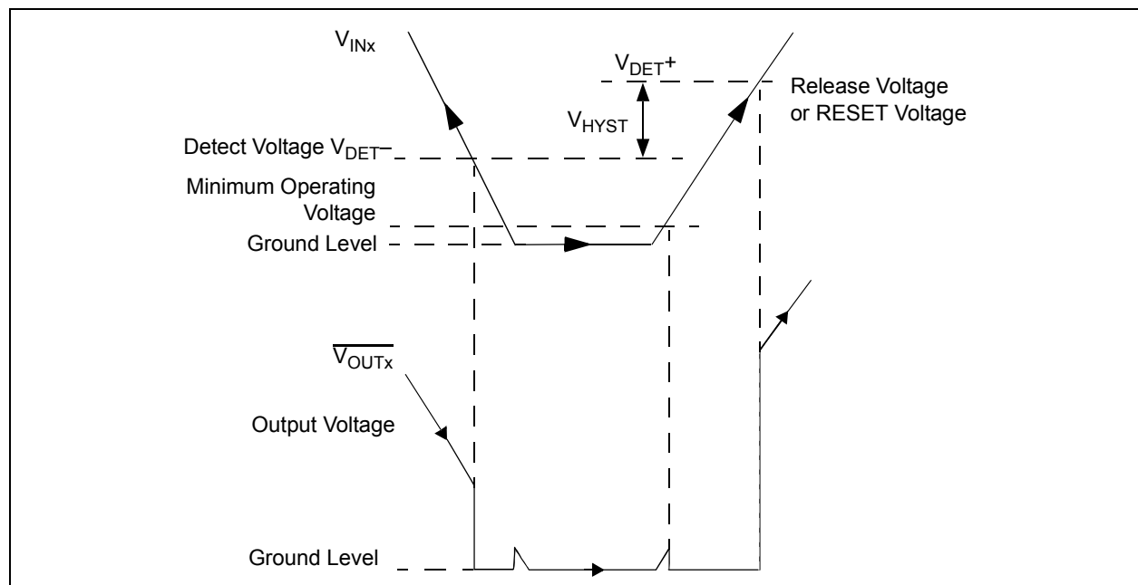
FIGURE 3-1: Timing Diagram.
