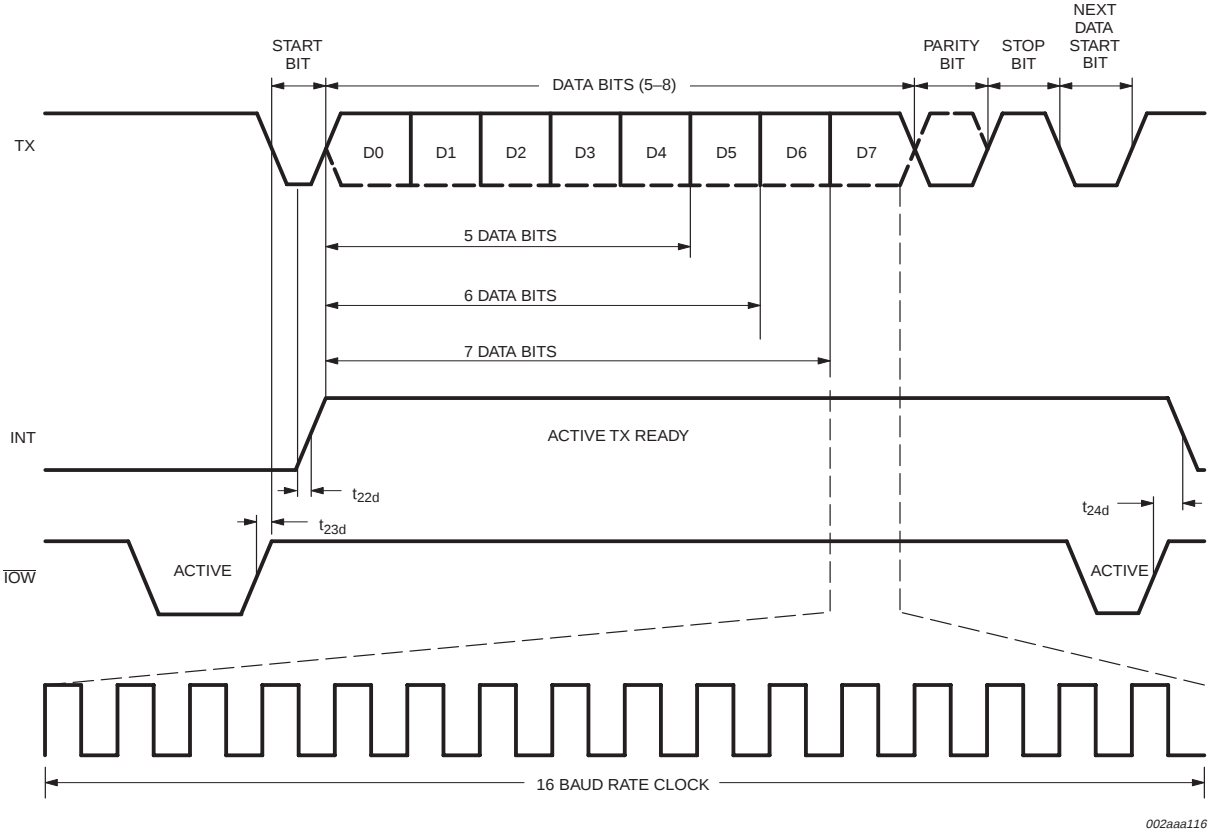
Fig 15. Transmit timing.
