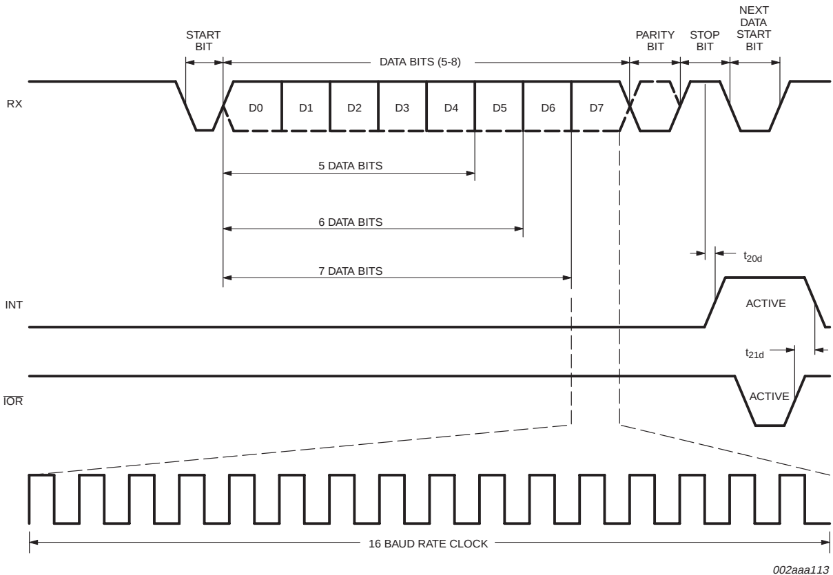
Fig 12. Receive timing.
