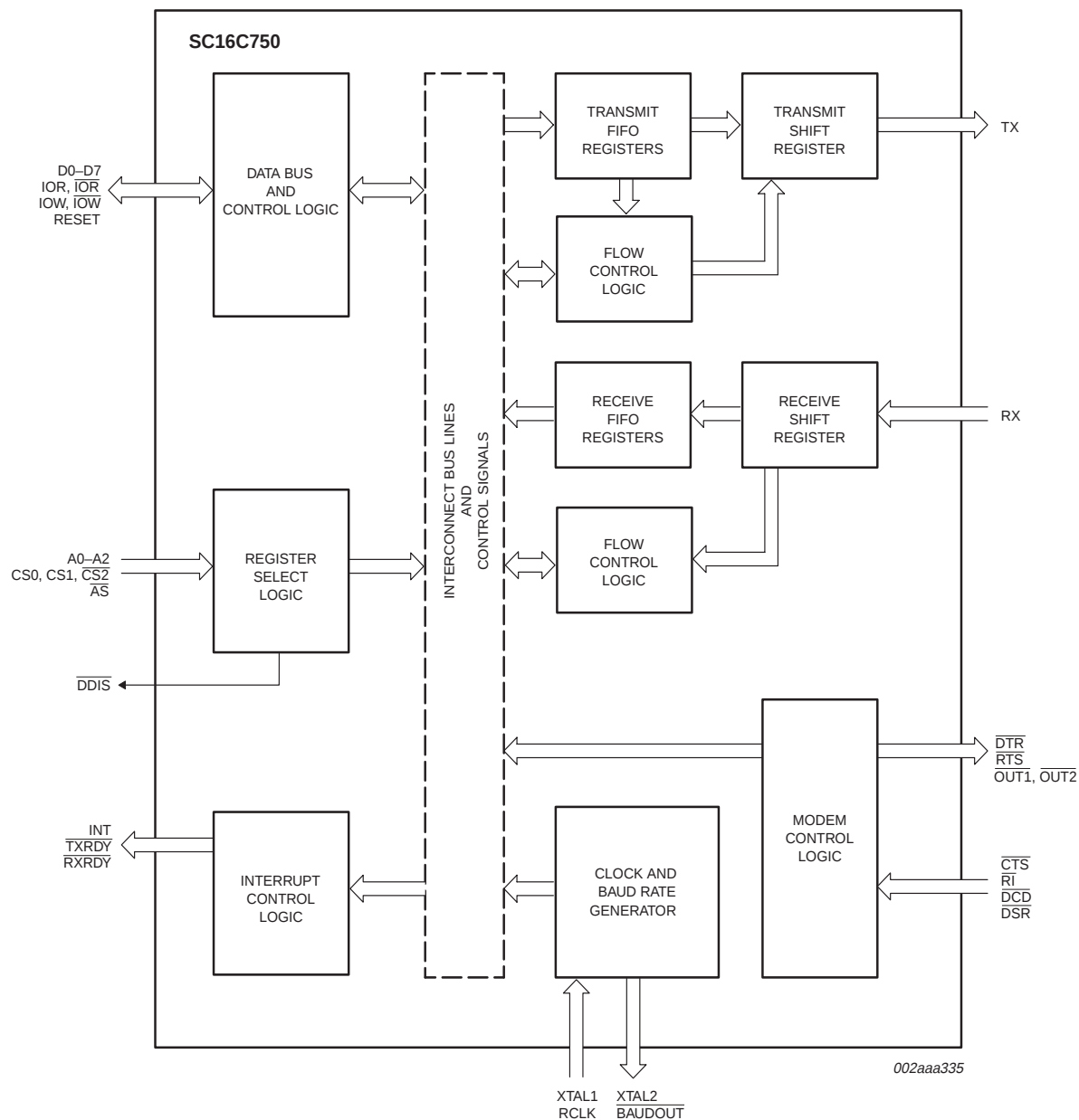
Fig 1. Block diagram.
